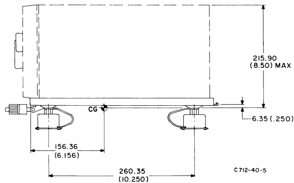
Figure 1-6. 51S-1B Receiver, Outline and Mounting Dimensions with 350D-5 Base Shockmount
