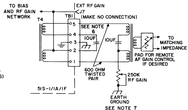
D. 600 OHM BAL 2-WIRE CONNECTIONS WITH REMOTE RF GAIN
